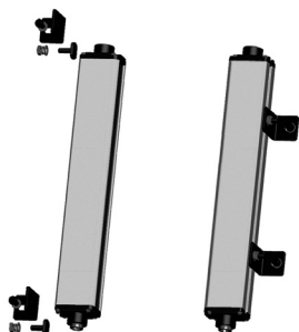
7.5 T型槽侧装 (TC)
