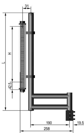
7.5 T型槽侧装 (TC)
